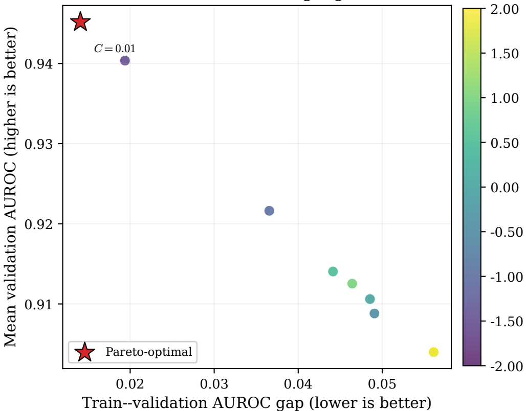
(a) Linear soft-margin grid
