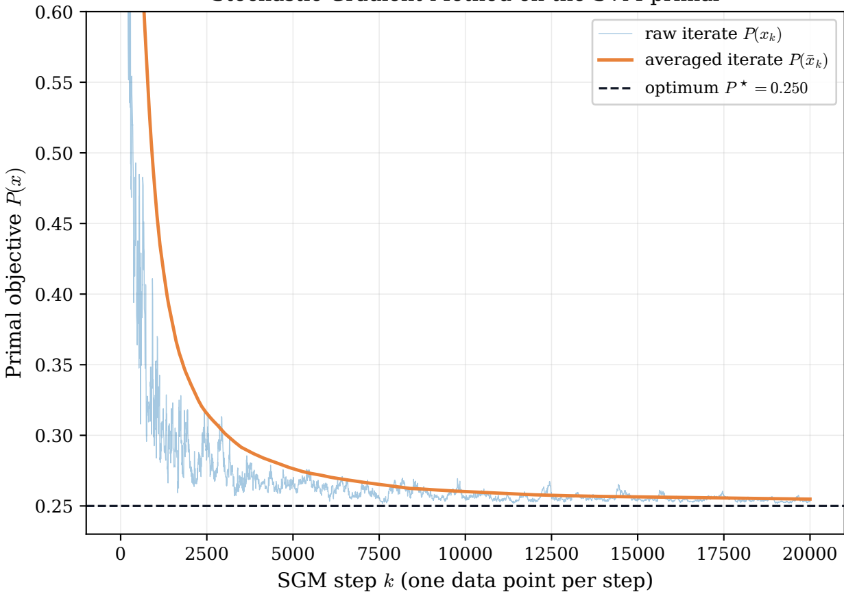
Stochastic Gradient Method on the SVM primal
