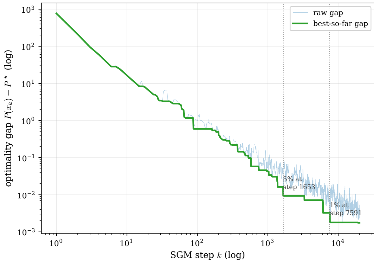
Convergence: steps to reach the optimum
