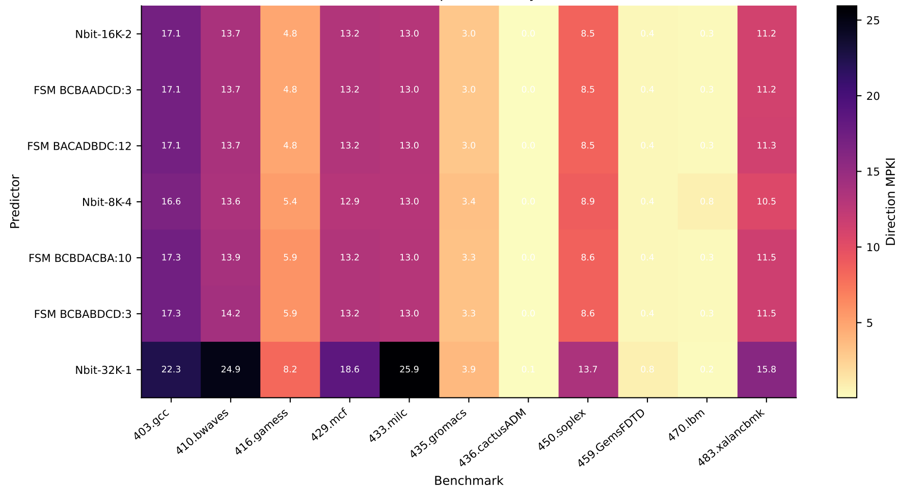
5.3 Fixed 32K-bit predictors by benchmark
