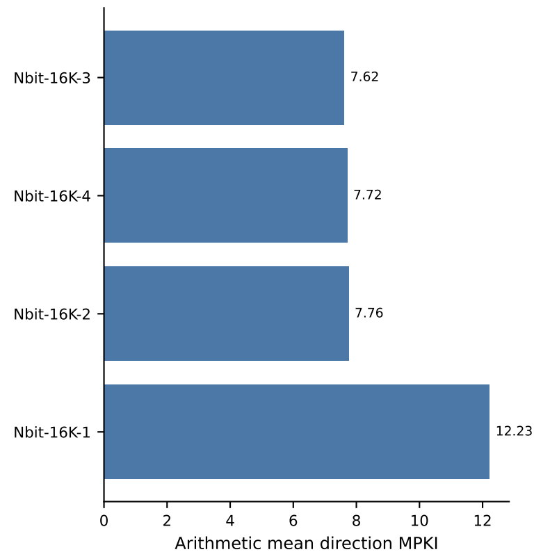
Fixed 16K entries
