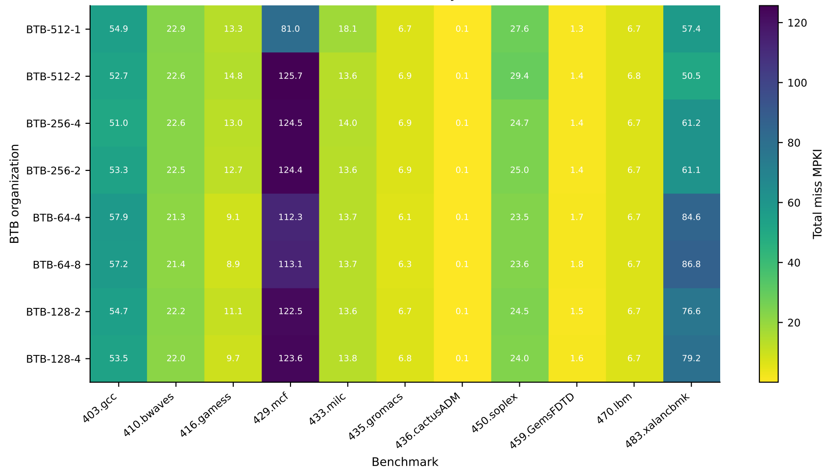
5.4 BTB total miss MPKI by benchmark
