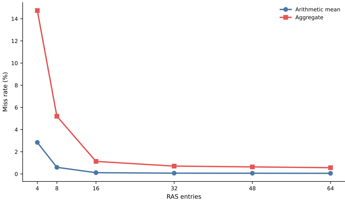
5.5 RAS miss rate versus stack entries
