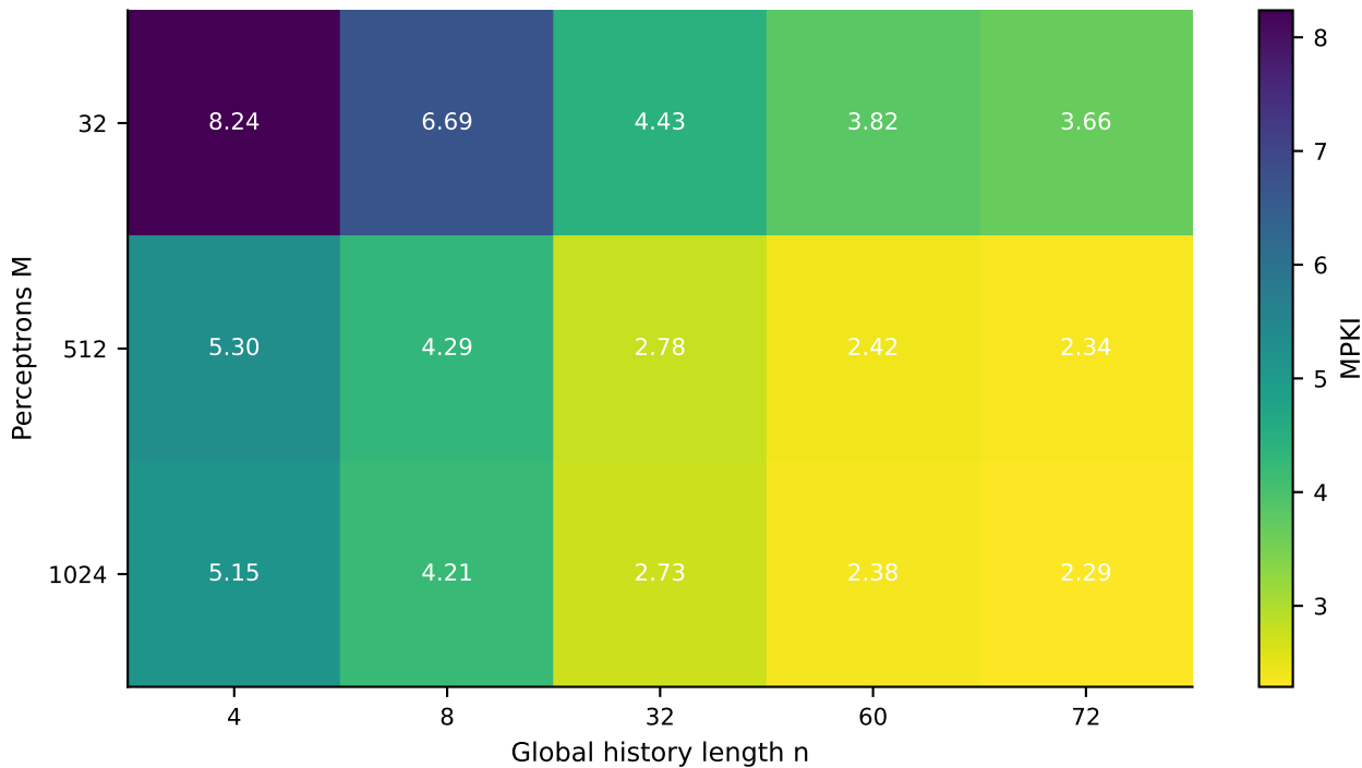
5.6.1 Perceptron arithmetic mean direction MPKI
