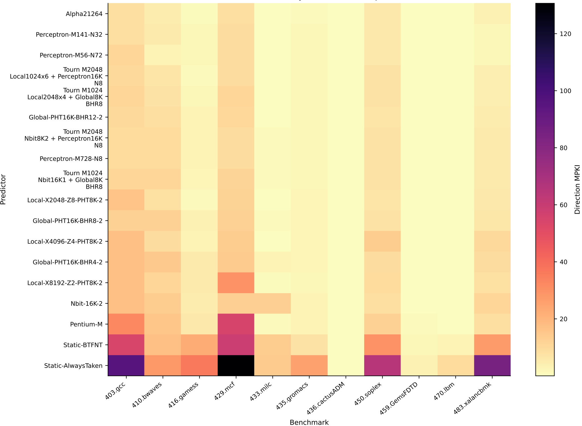
5.6.2 Direction MPKI by benchmark and predictor
