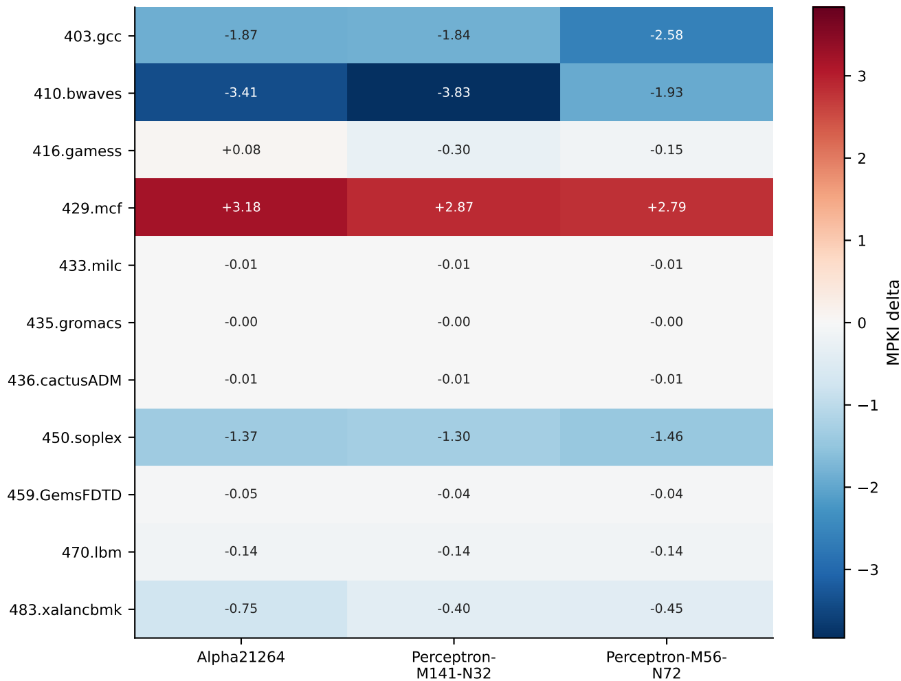
5.7 Ref - train direction MPKI delta
