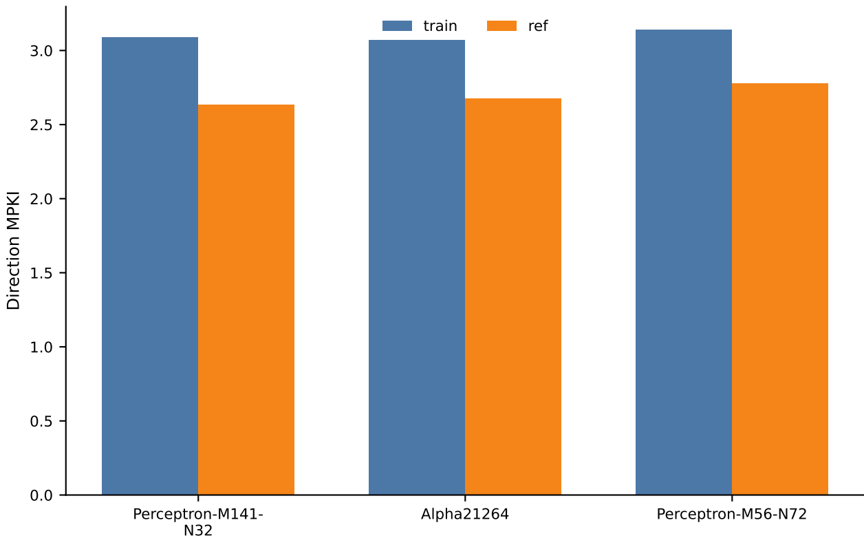
5.7 Train versus ref arithmetic mean MPKI
