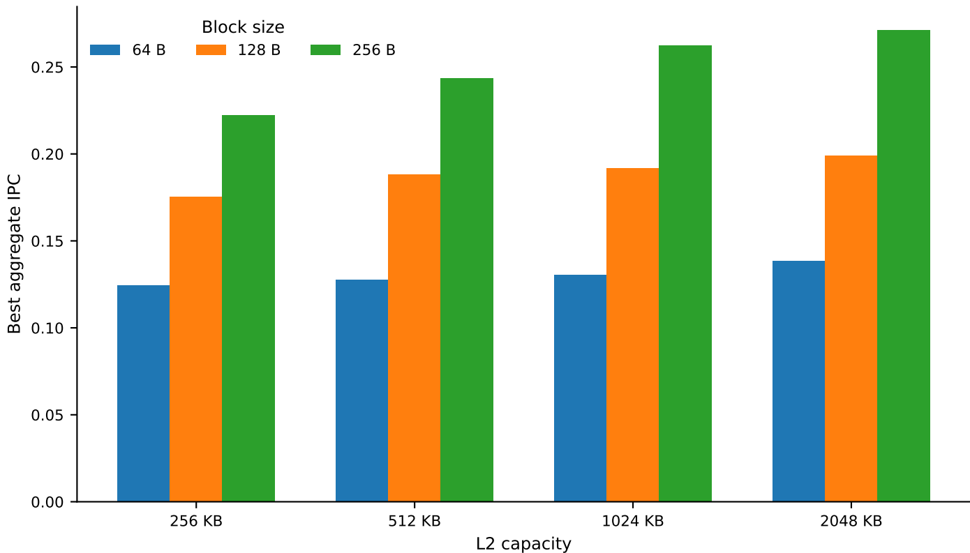
4.2 Block-size sensitivity using best associativity per capacity
