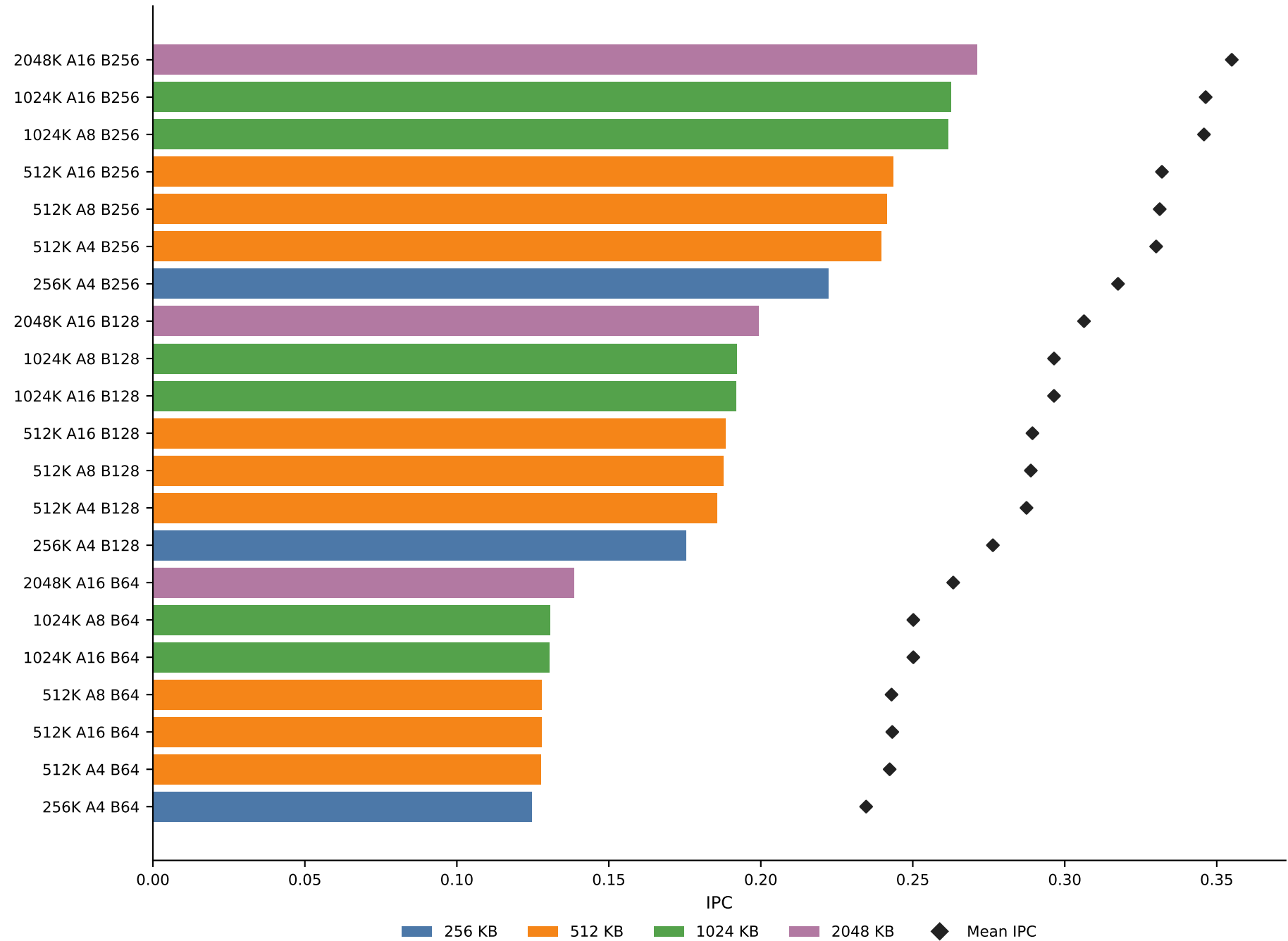
4.2 L2 configurations ranked by aggregate IPC
