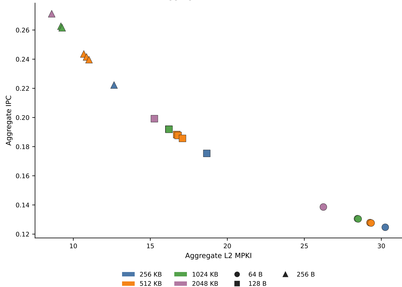
4.2 Aggregate IPC versus L2 MPKI
