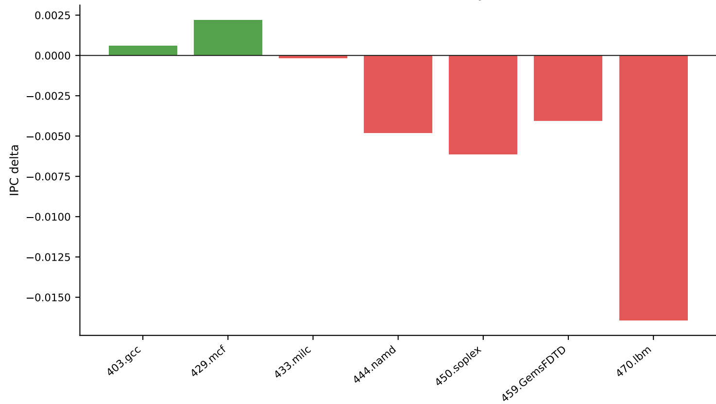
4.3 Random minus LRU mean IPC by benchmark
