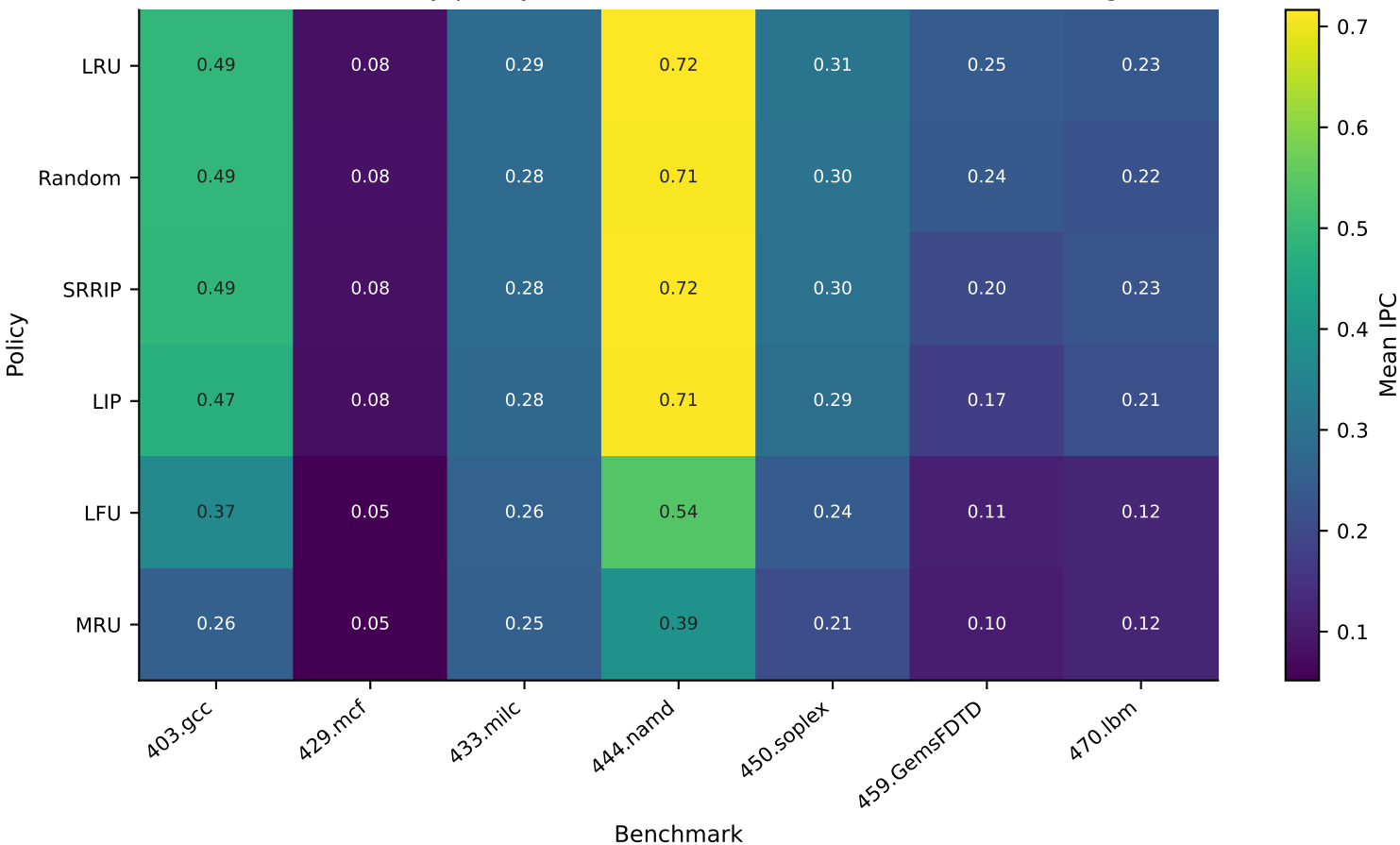
4.3 Mean IPC by policy and benchmark across selected L2 configs
