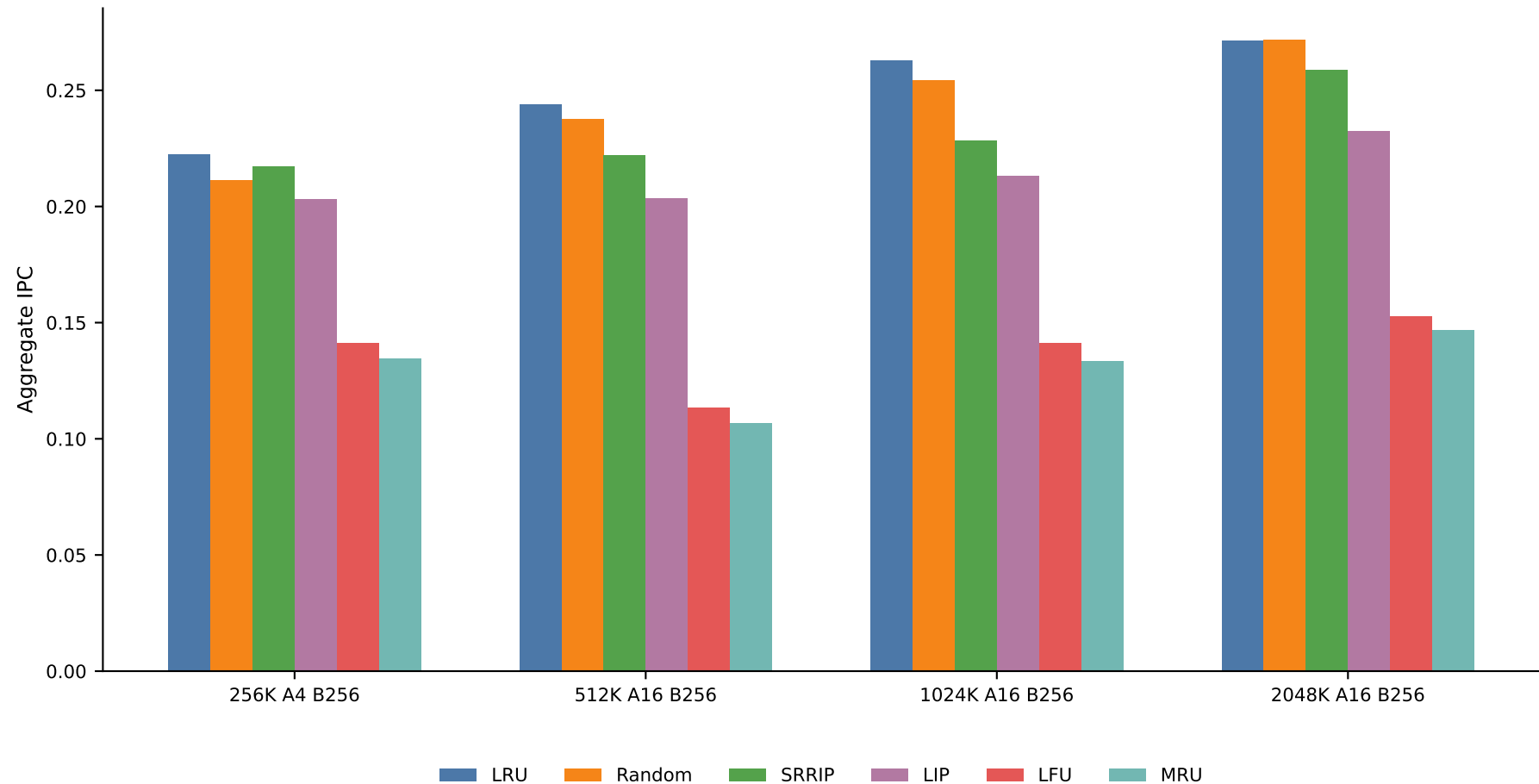
4.3 Aggregate IPC by replacement policy and selected L2 config
