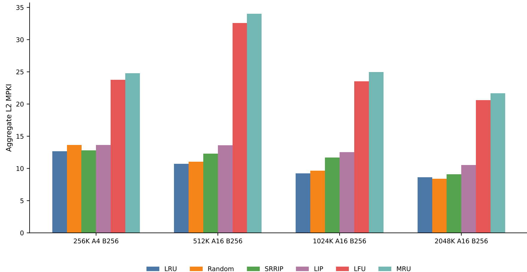
4.3 Aggregate L2 MPKI by replacement policy and selected L2 config
