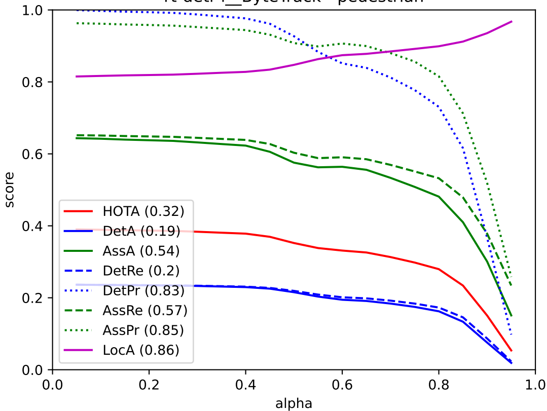
rt-detr-l__ByteTrack - pedestrian
