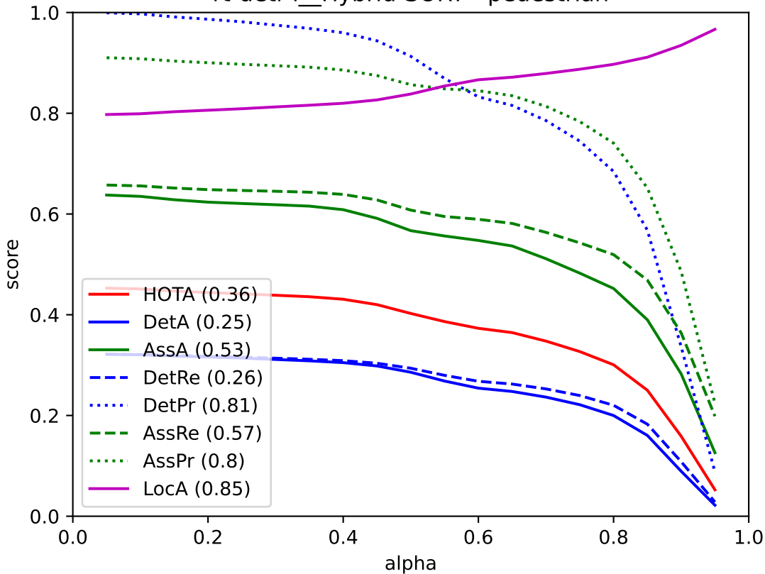
rt-detr-l__Hybrid-SORT - pedestrian
