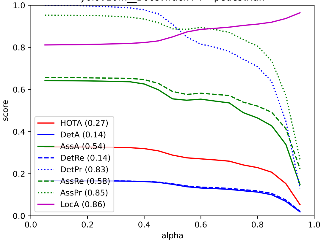
yolov10m_BoostTrack++ - pedestrian
