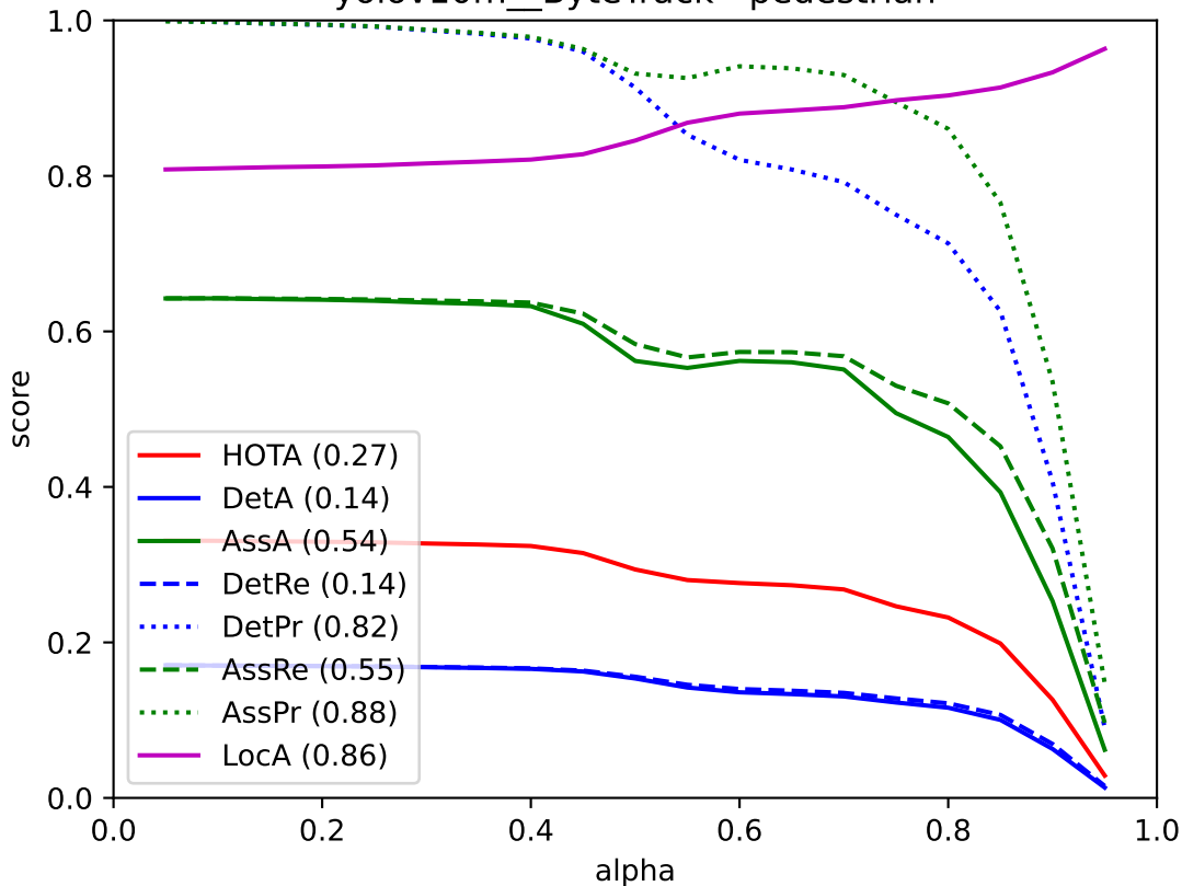
yolov10m__ByteTrack - pedestrian
