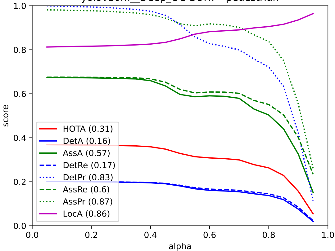
yolov10m_Deep_OC-SORT - pedestrian
