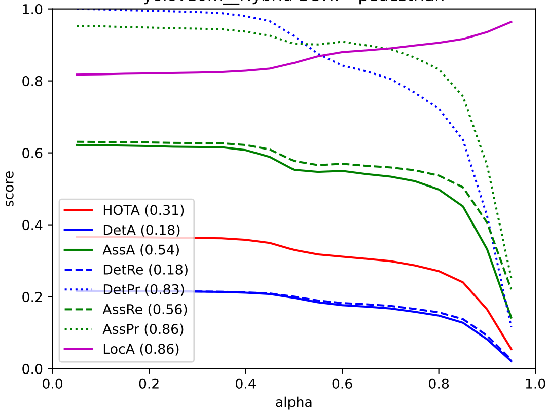
yolov10m__Hybrid-SORT - pedestrian
