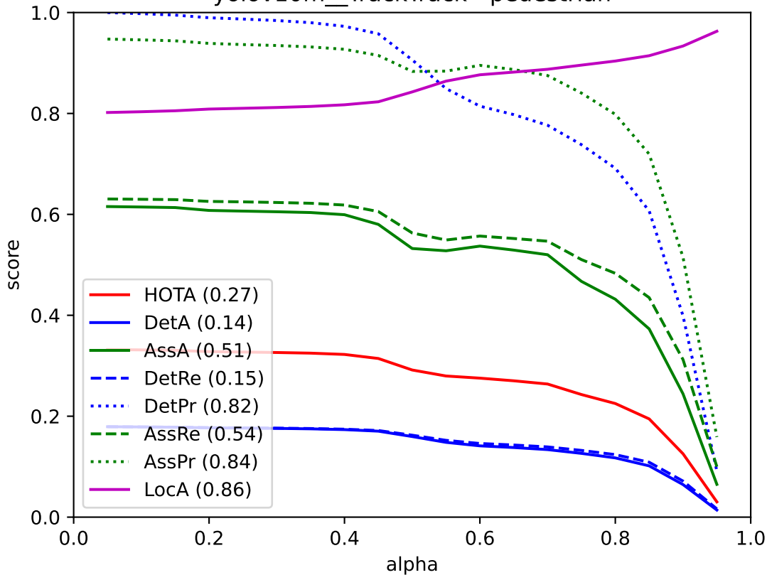
yolov10m_TrackTrack - pedestrian
