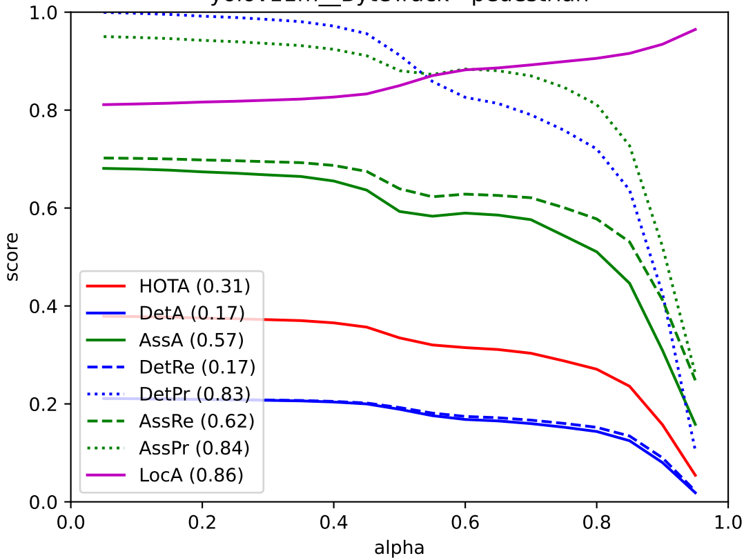
yolov11m_ByteTrack - pedestrian
