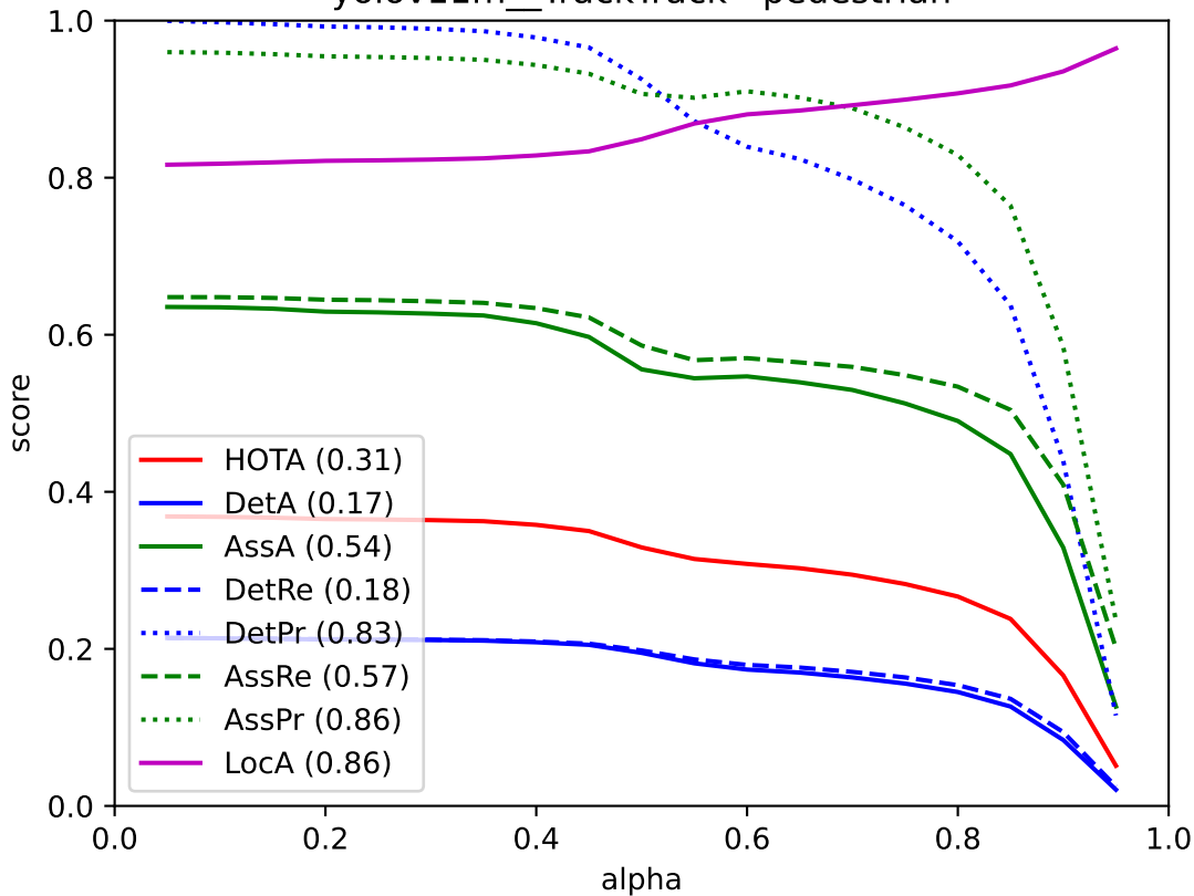
yolov11m_TrackTrack - pedestrian
