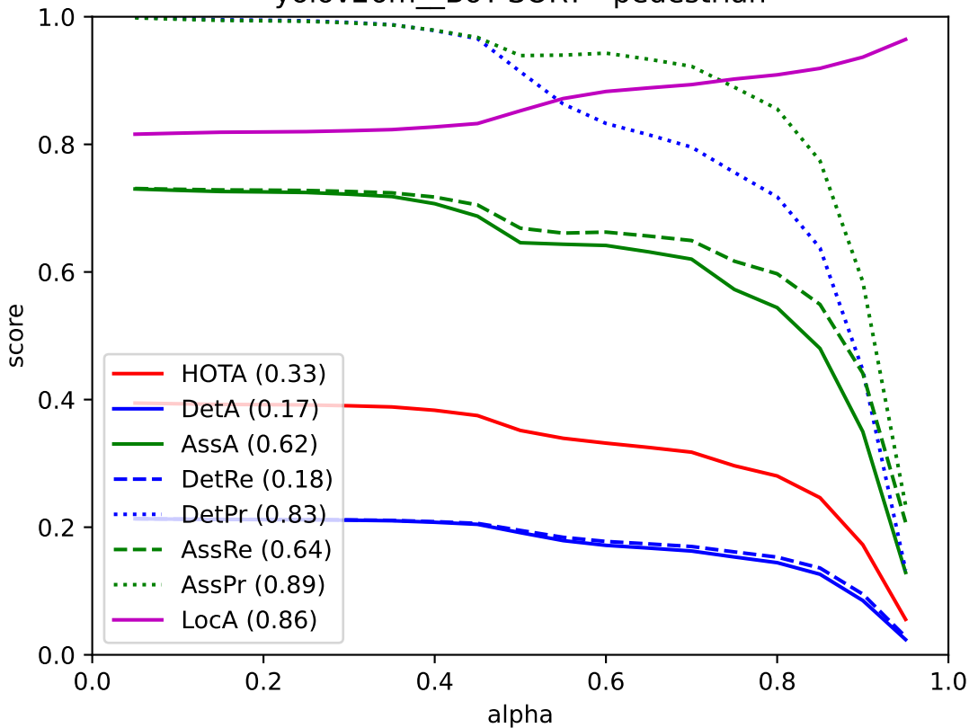
yolov26m__BoT-SORT - pedestrian
