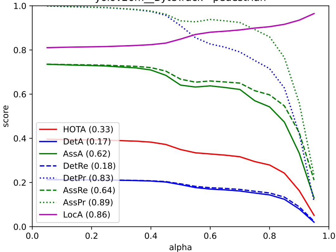
yolov26m__ByteTrack - pedestrian
