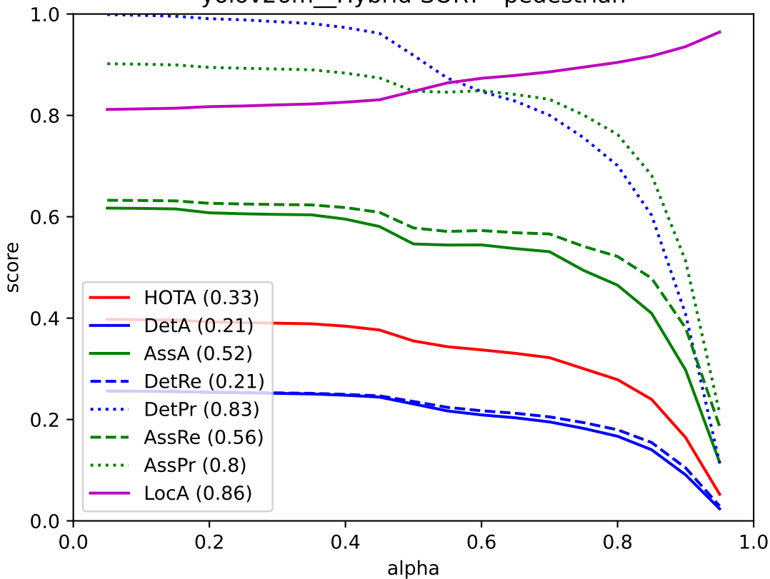
yolov26m__Hybrid-SORT - pedestrian
