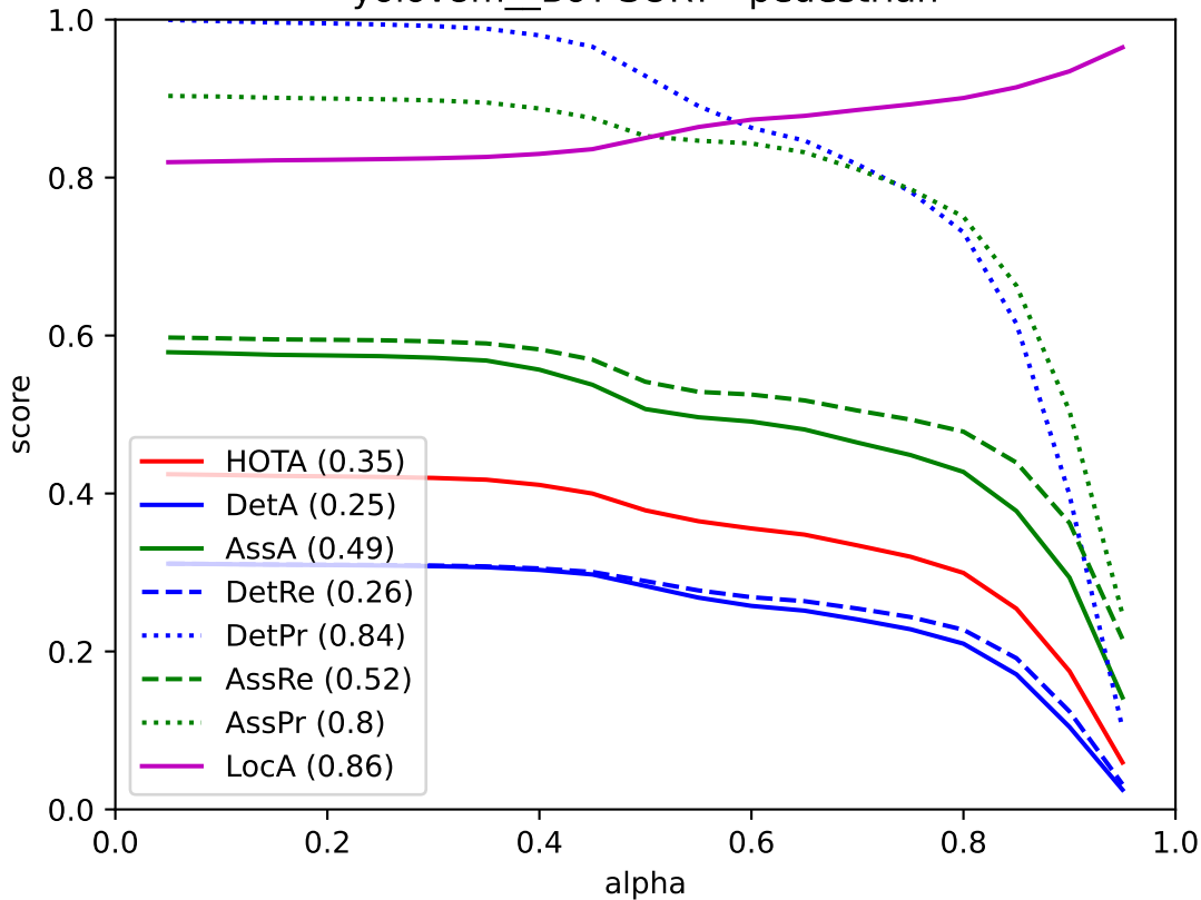
yolov8m_BoT-SORT - pedestrian
