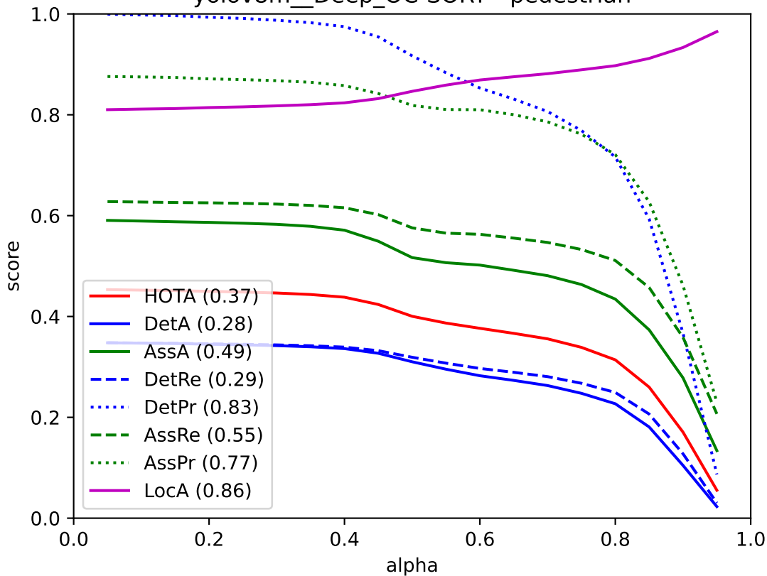
yolov8m_Deep_OC-SORT - pedestrian
