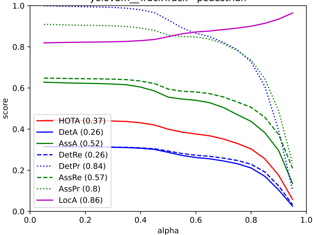
yolov8m_TrackTrack - pedestrian
