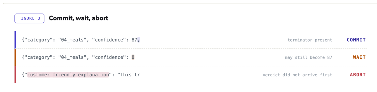
Figure 3 — Commit, wait, abort. The middle buffer waits because the next chunk may turn 8 into 87. Image by the author.
