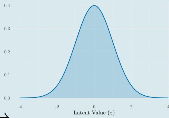
Base Distribution Latent Space: \mathcal{Z} \sim \mathcal{N}(0, 1)
