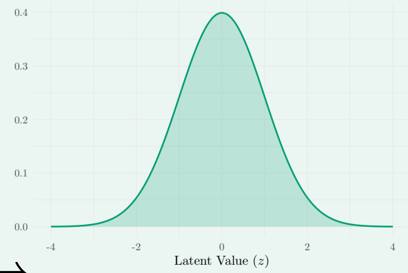
Base Distribution Latent Space: \mathcal{Z} \sim \mathcal{N}(0, 1)
