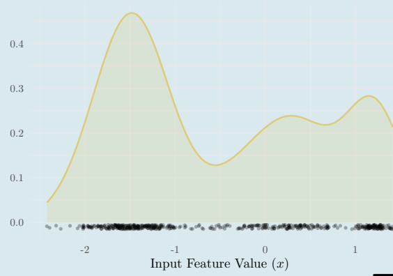
Input Data Distribution Observed Space ( \mathcal{X} )
