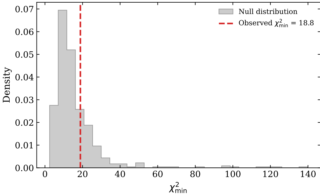
Truncated Gaussian ( p = 0.244 )
