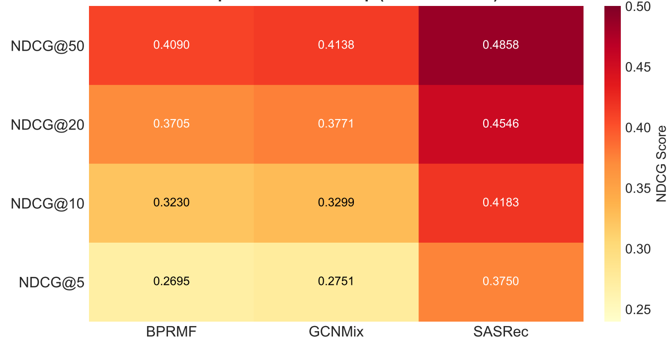
Dev Split - NDCG Heatmap (MovieLens-1M)
