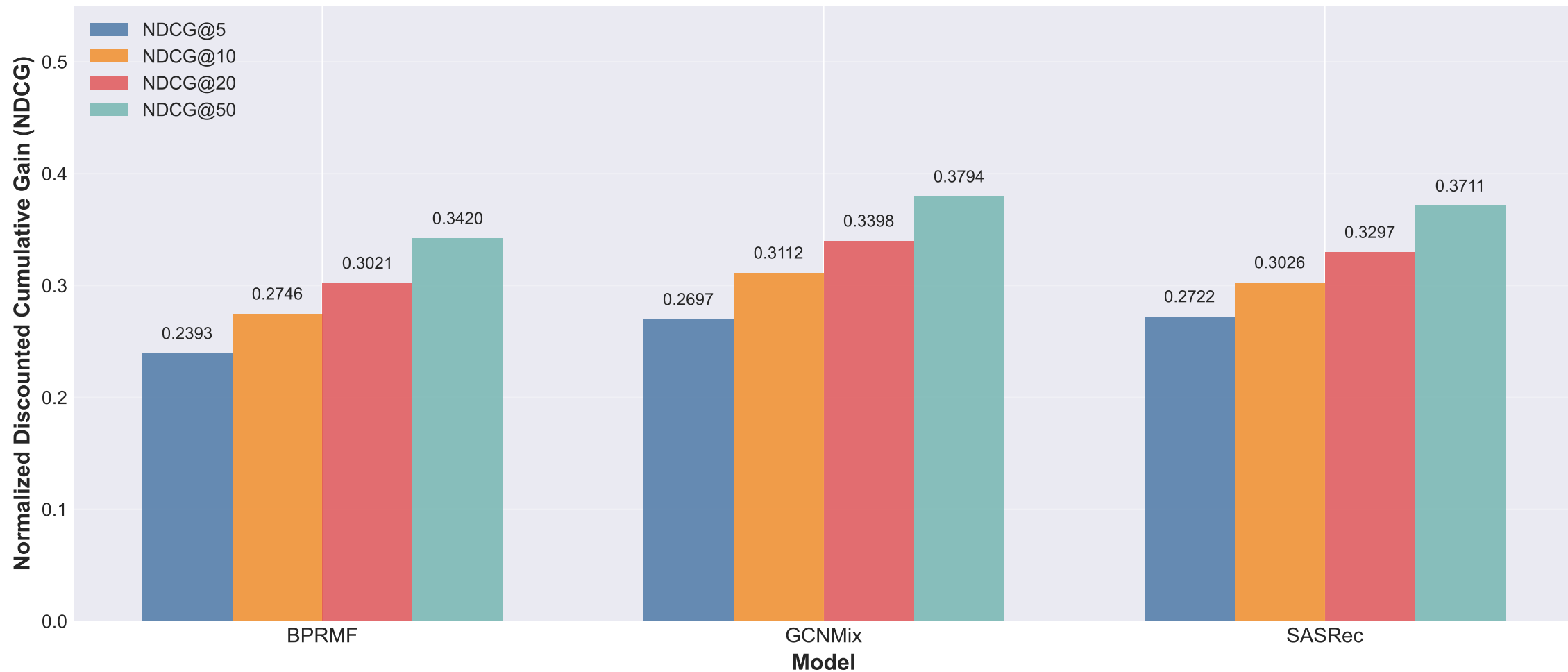
Test Split - NDCG Metric Comparison (Grocery & Gourmet Food)
