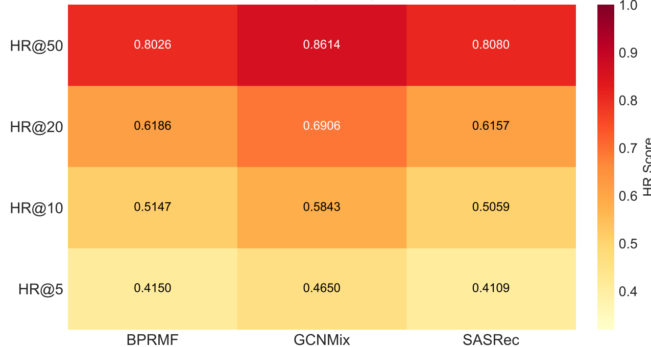
Dev Split - HR Heatmap (Grocery &amp; Gourmet Food)
