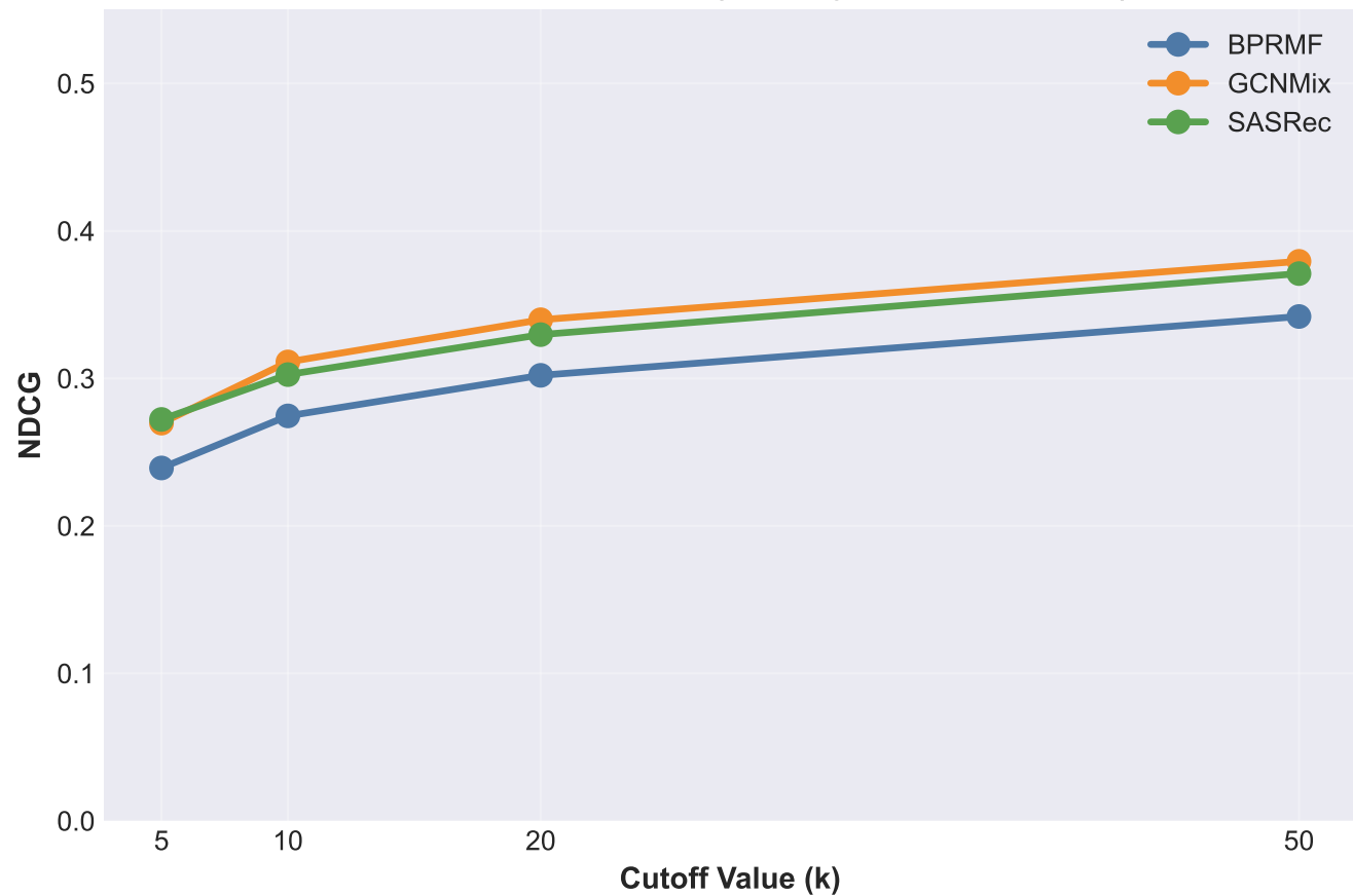
Test Split - NDCG Curve (Grocery & Gourmet Food)
