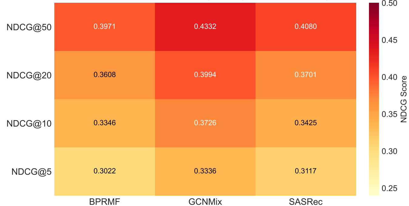
Dev Split - NDCG Heatmap (Grocery &amp; Gourmet Food)
