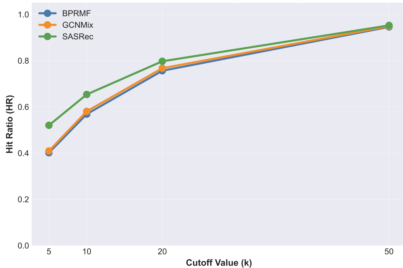
Dev Split - HR Curve (MovieLens-1M)
