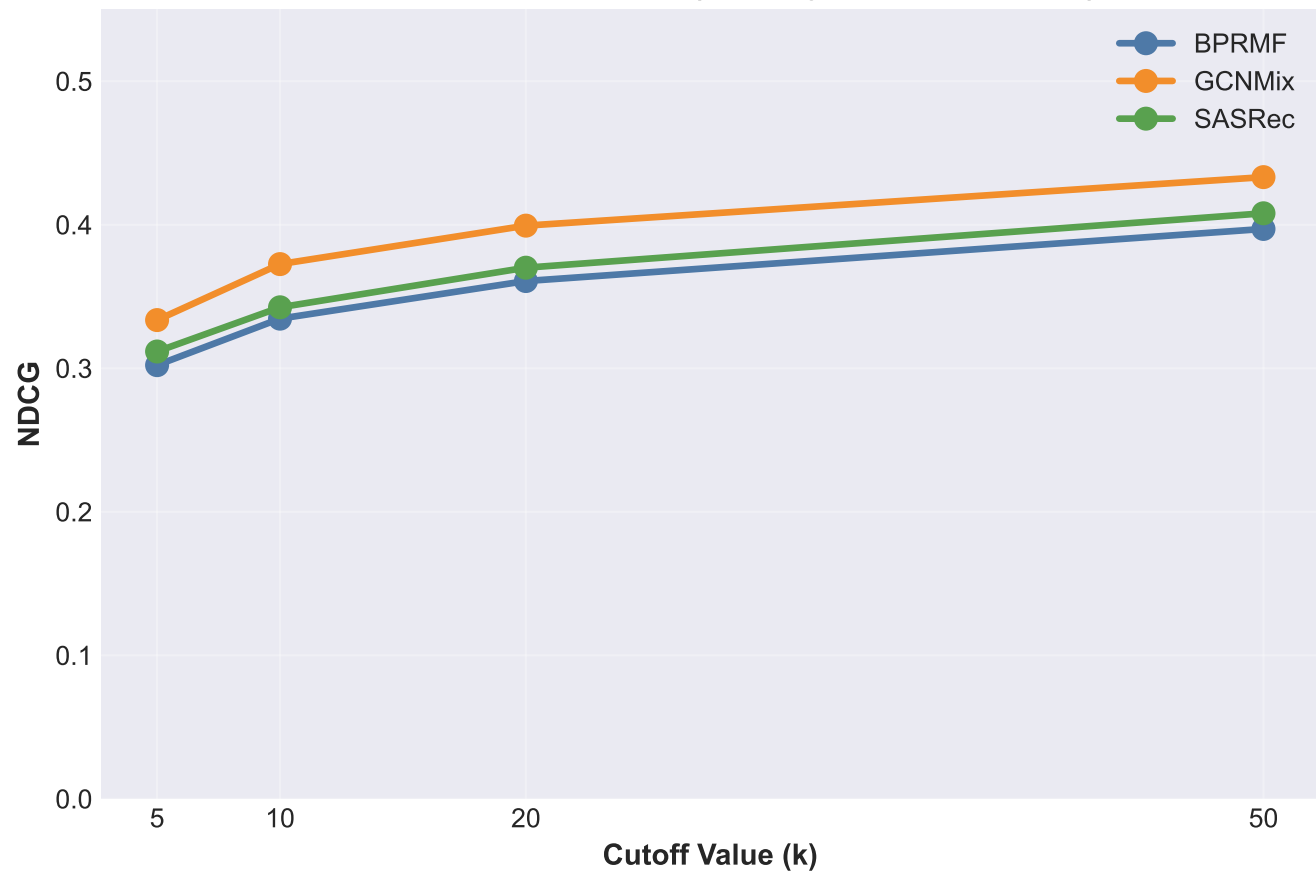
Dev Split - NDCG Curve (Grocery & Gourmet Food)
