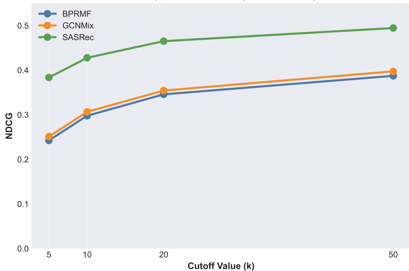
Test Split - NDCG Curve (MovieLens-1M)
