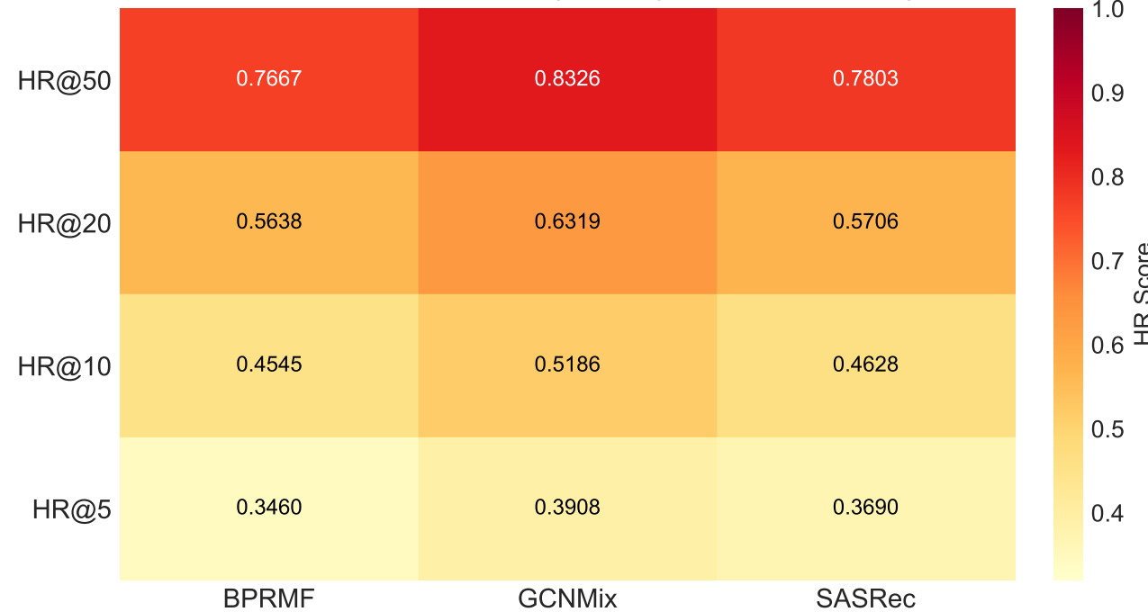
Test Split - HR Heatmap (Grocery & Gourmet Food)
