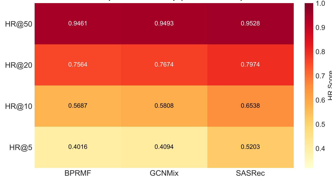
Dev Split - HR Heatmap (MovieLens-1M)
