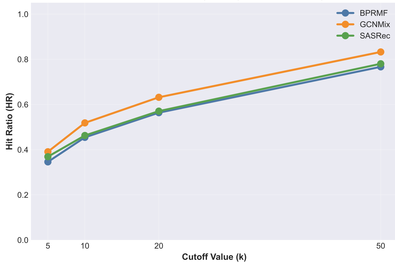
Test Split - HR Curve (Grocery & Gourmet Food)
