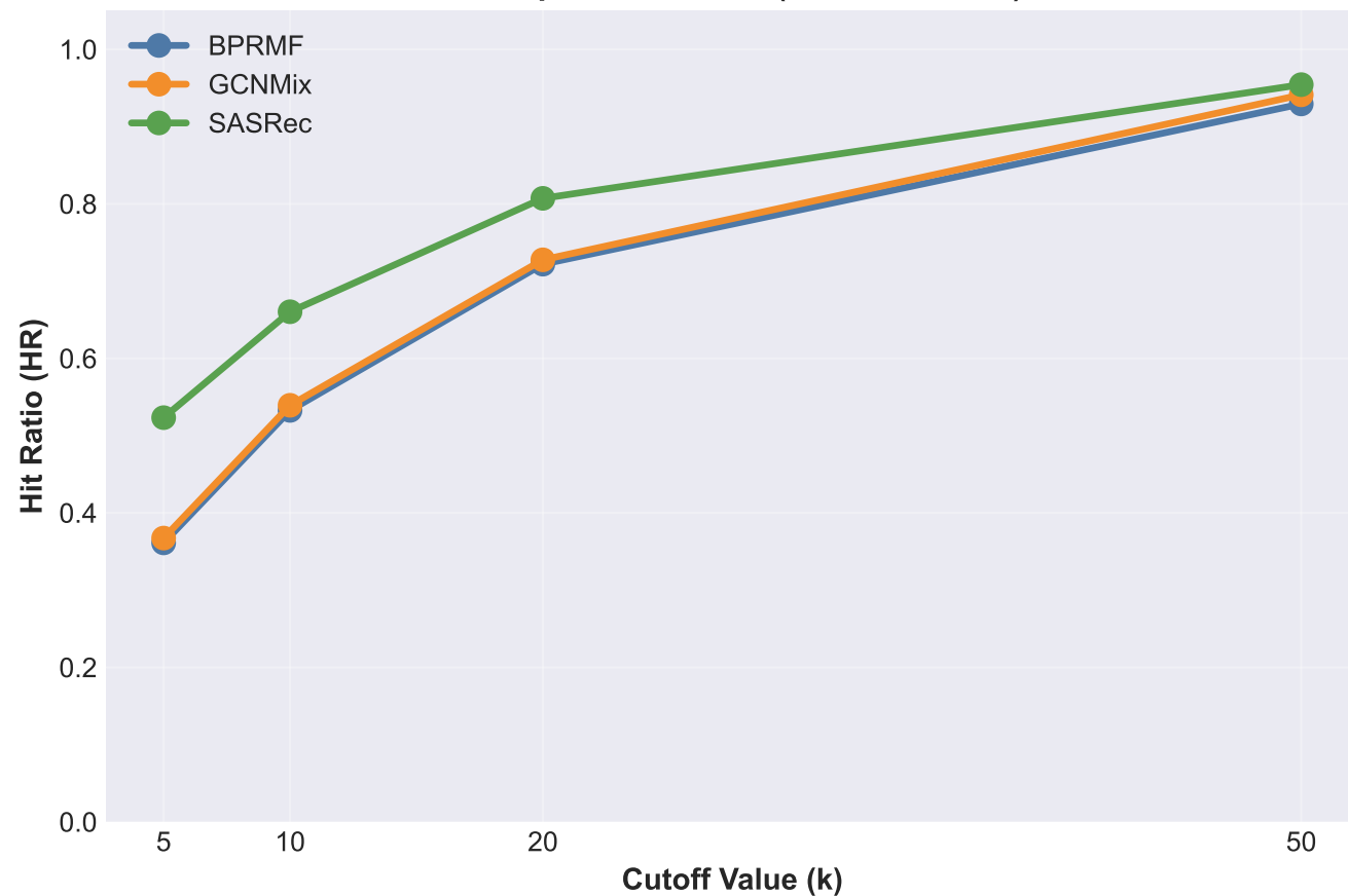
Test Split - HR Curve (MovieLens-1M)
