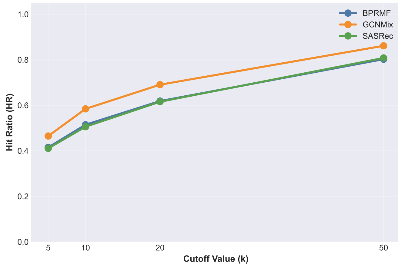
Dev Split - HR Curve (Grocery & Gourmet Food)
