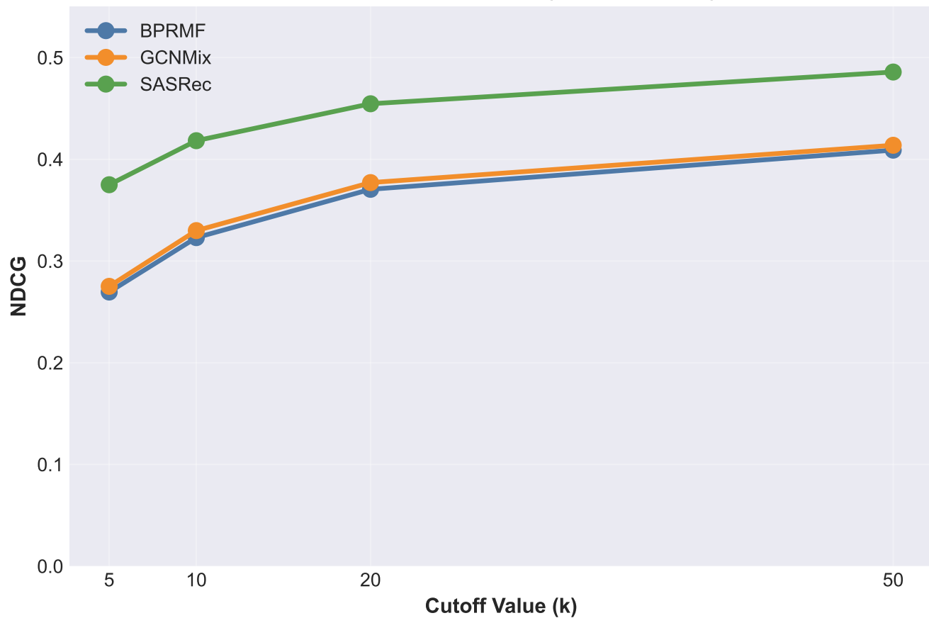
Dev Split - NDCG Curve (MovieLens-1M)
