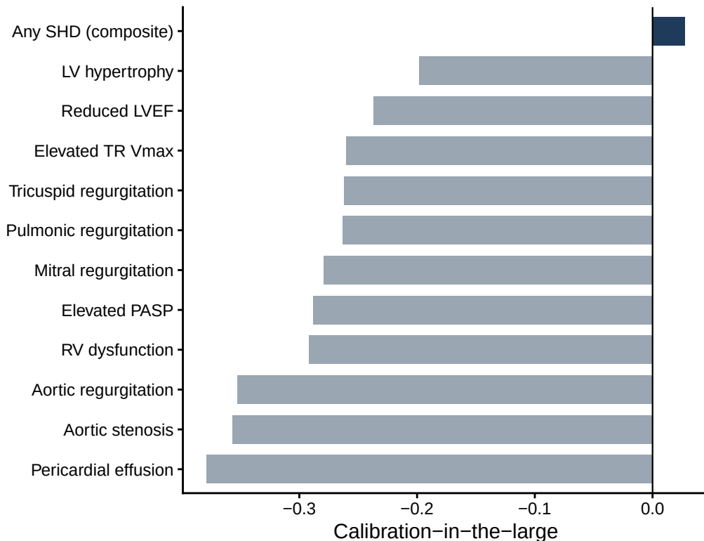
Per-condition over-prediction
