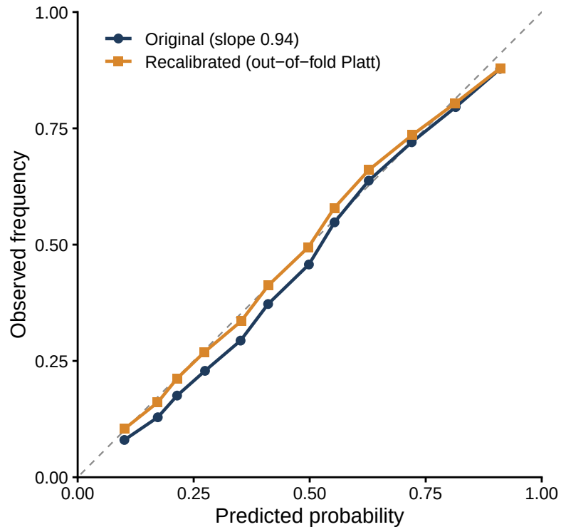
Any-SHD calibration
