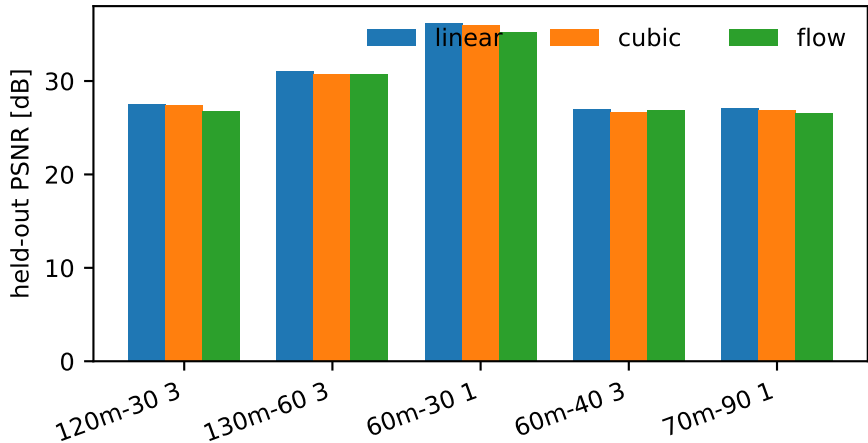
Interpolation on real thermal video (7.5 Hz, 4x)
