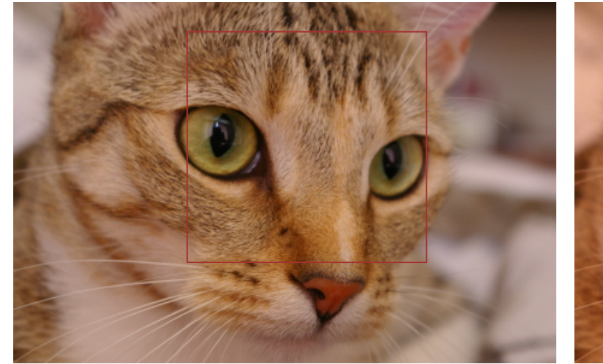
(a) Source
