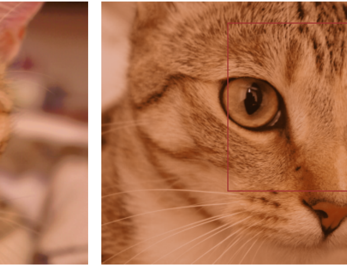
(f) Sinkhorn
