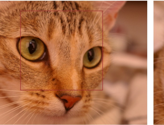
(c) AdaIN
