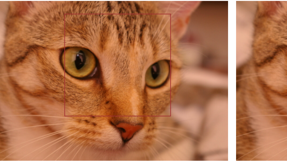
(b) Reference
