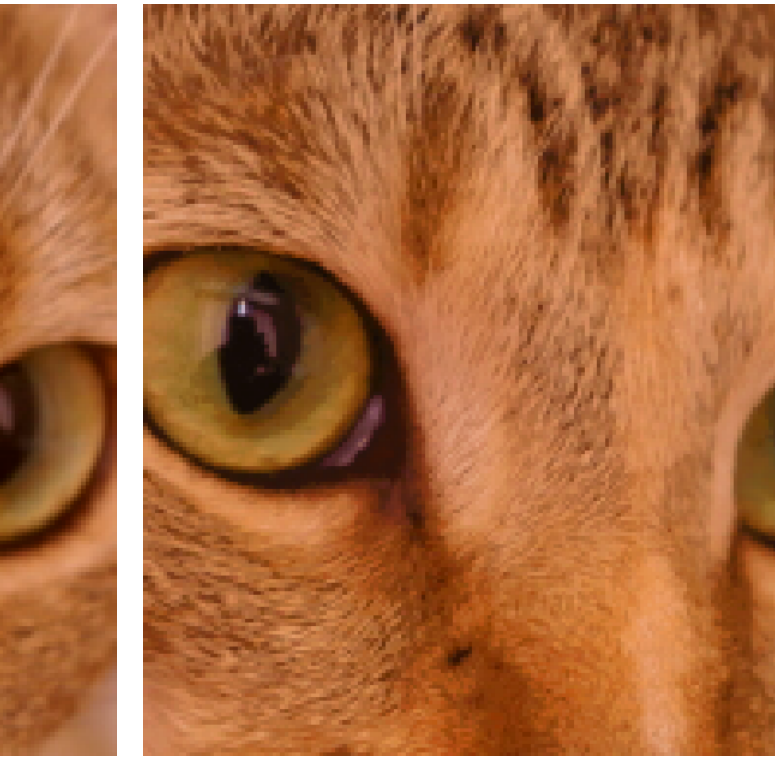
(e) Sliced OT
