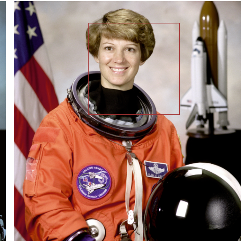
(b) Reference
