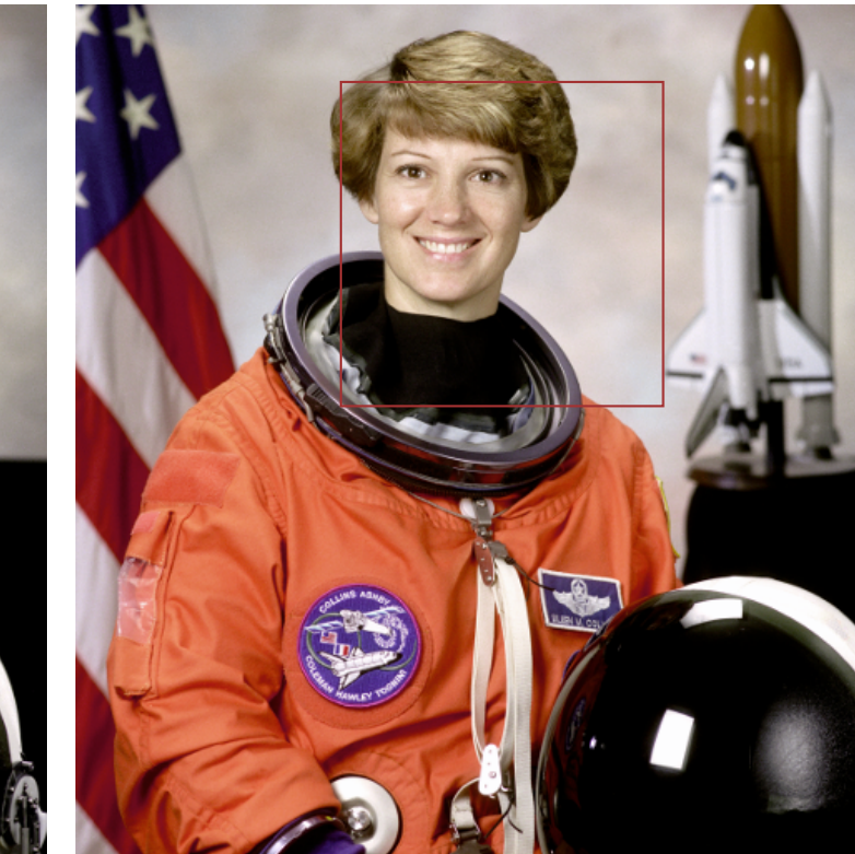
(c) AdaIN
