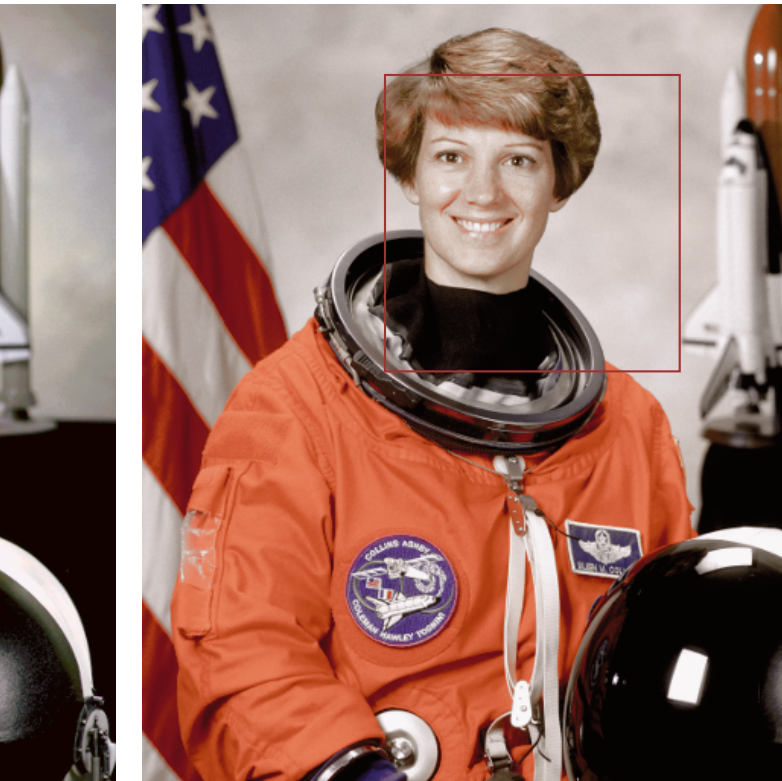
(f) Sinkhorn
