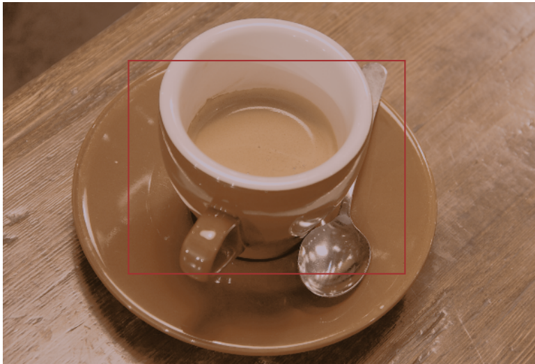
(e) Sinkhorn
