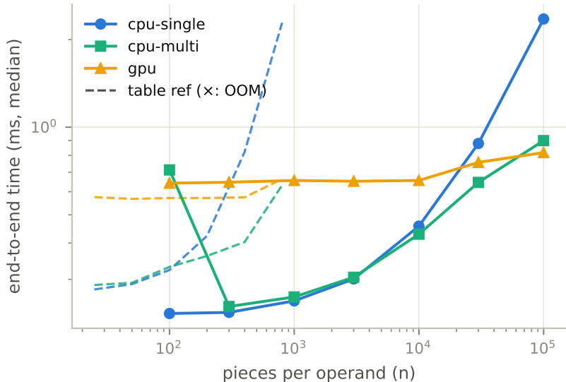
box_search (xy,xy->xy)
