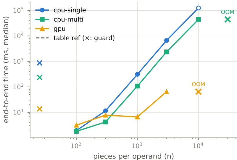
triple_contract_ii (ij,ik,kj-&gt;ij)
