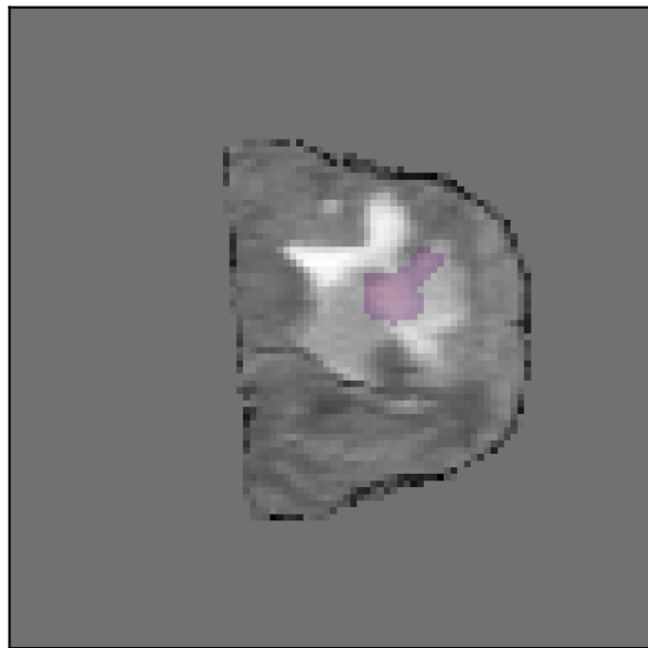
(b) Grad-CAM
