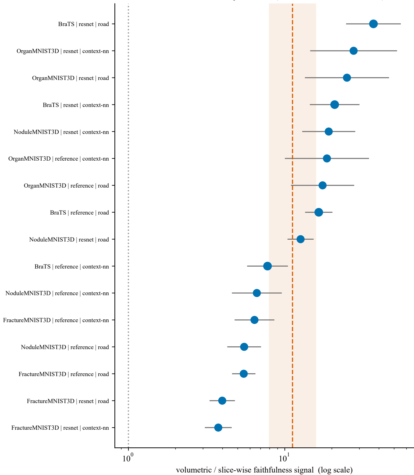
Slice illusion across datasets: pooled 11.2x (95% CI 8.0 to 15.8; I2=96%, k=16)
