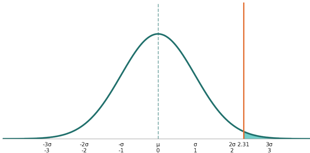
t-Distribution: Right-Tailed Test ( df \approx 37 )
