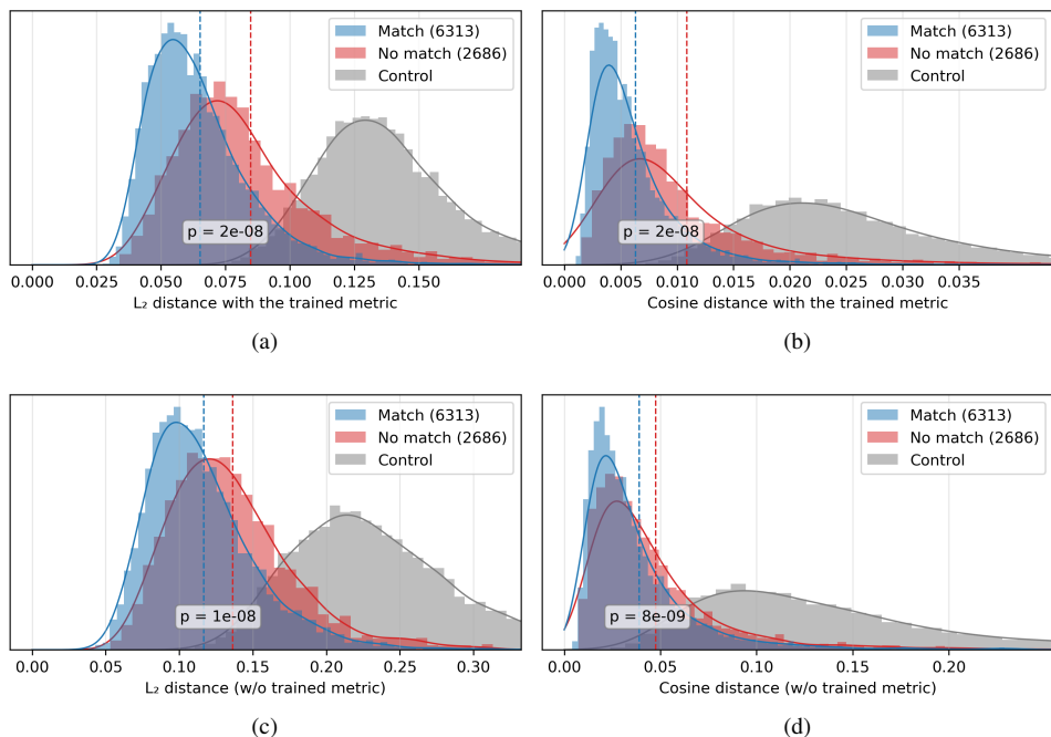
Figure 9: The distance between the “chemembedding” predicted by the model at checkpoint (17.7) and the “chemembedding” of the canonical reference SMILES, stratified by whether there is a top-10 exact structure match. As control, the distances between all the reference SMILES are also shown. Left vs right: measured in dimension-normalized L_2 -norm \frac{1}{\sqrt{n}} \|\cdot\|_2 vs measured using cosine distance ( 1 - \cos \angle ). Top vs bottom: the trainable metric-matrix from (10) is applied first vs omitted. The p-value shown is computed using the Cramér–von Mises test between the empirical data of “match” and “no match”.
