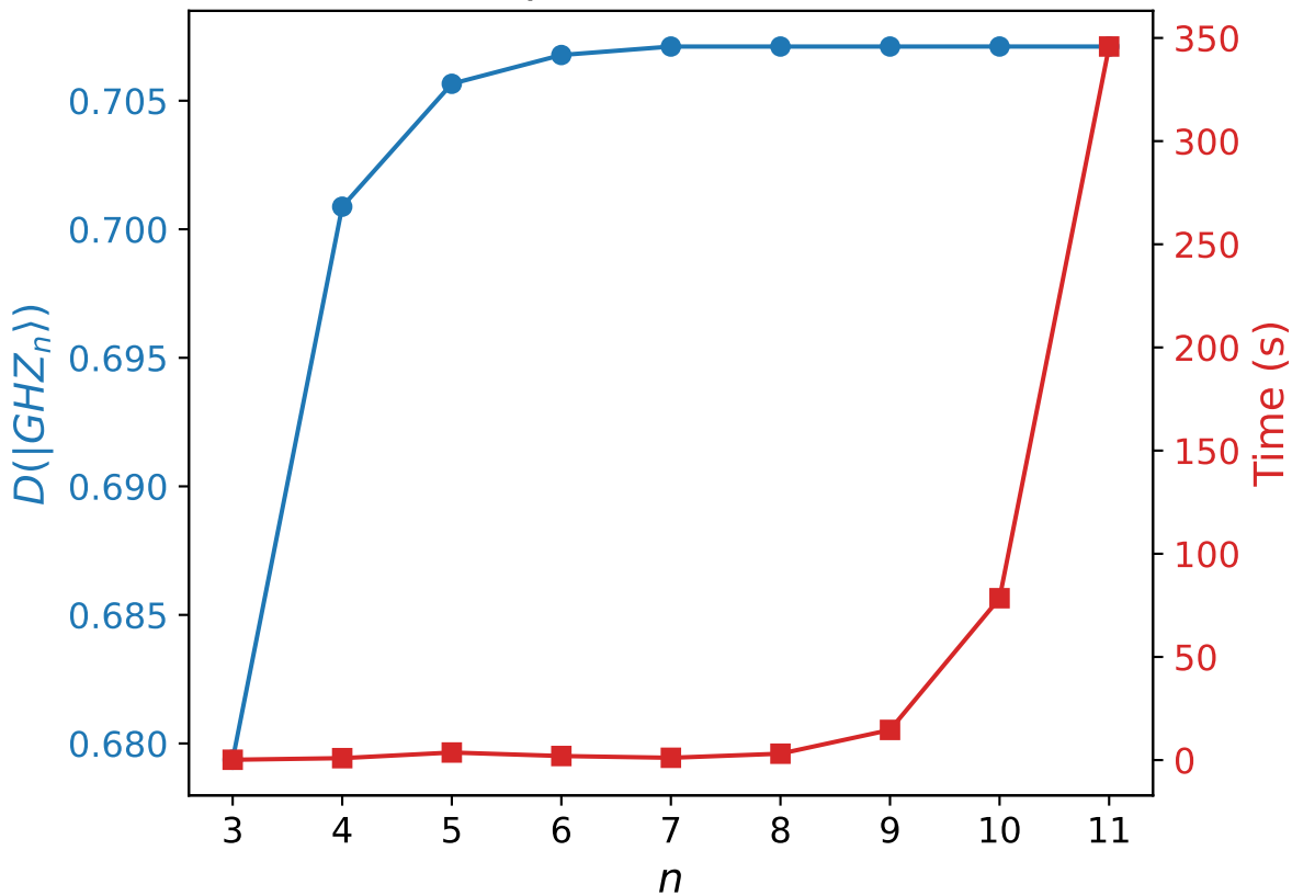
n -qubit GHZ state
