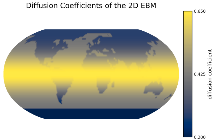
Figure 1: Diffusion coefficients
